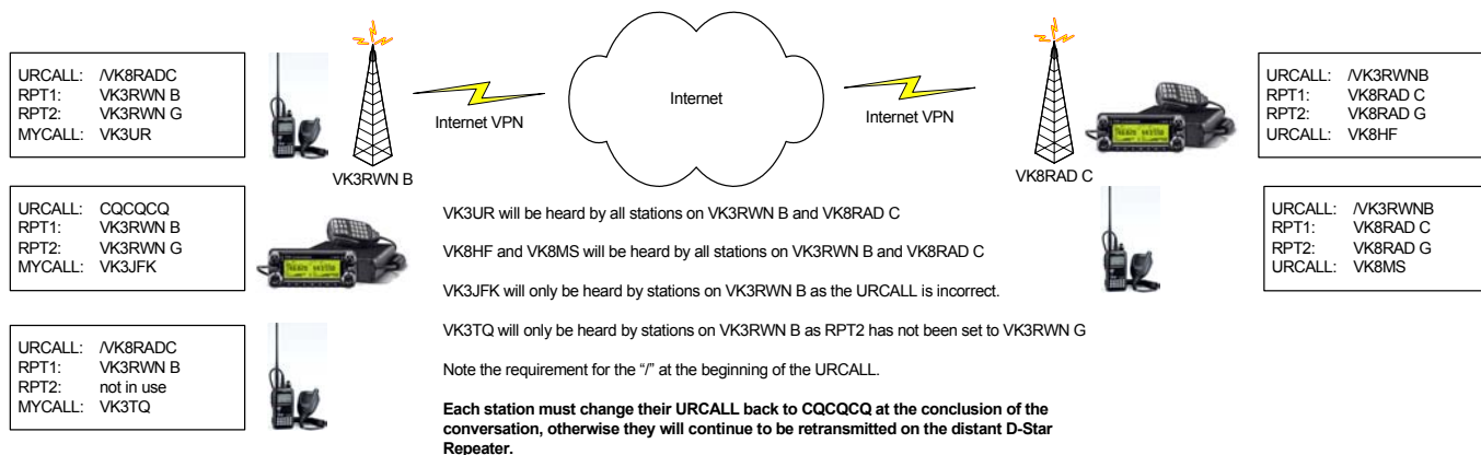
Figure 1: Example of Node Linking across D-Star
